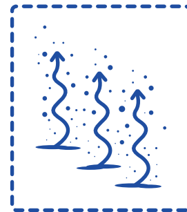
Evaporation
