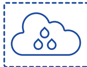
Condensation
