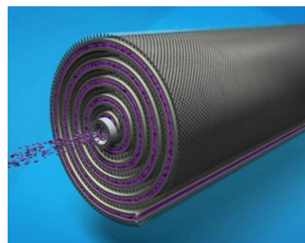
Spiral wound layers in a RO membrane module. The flow of water molecules is shown in purple.
