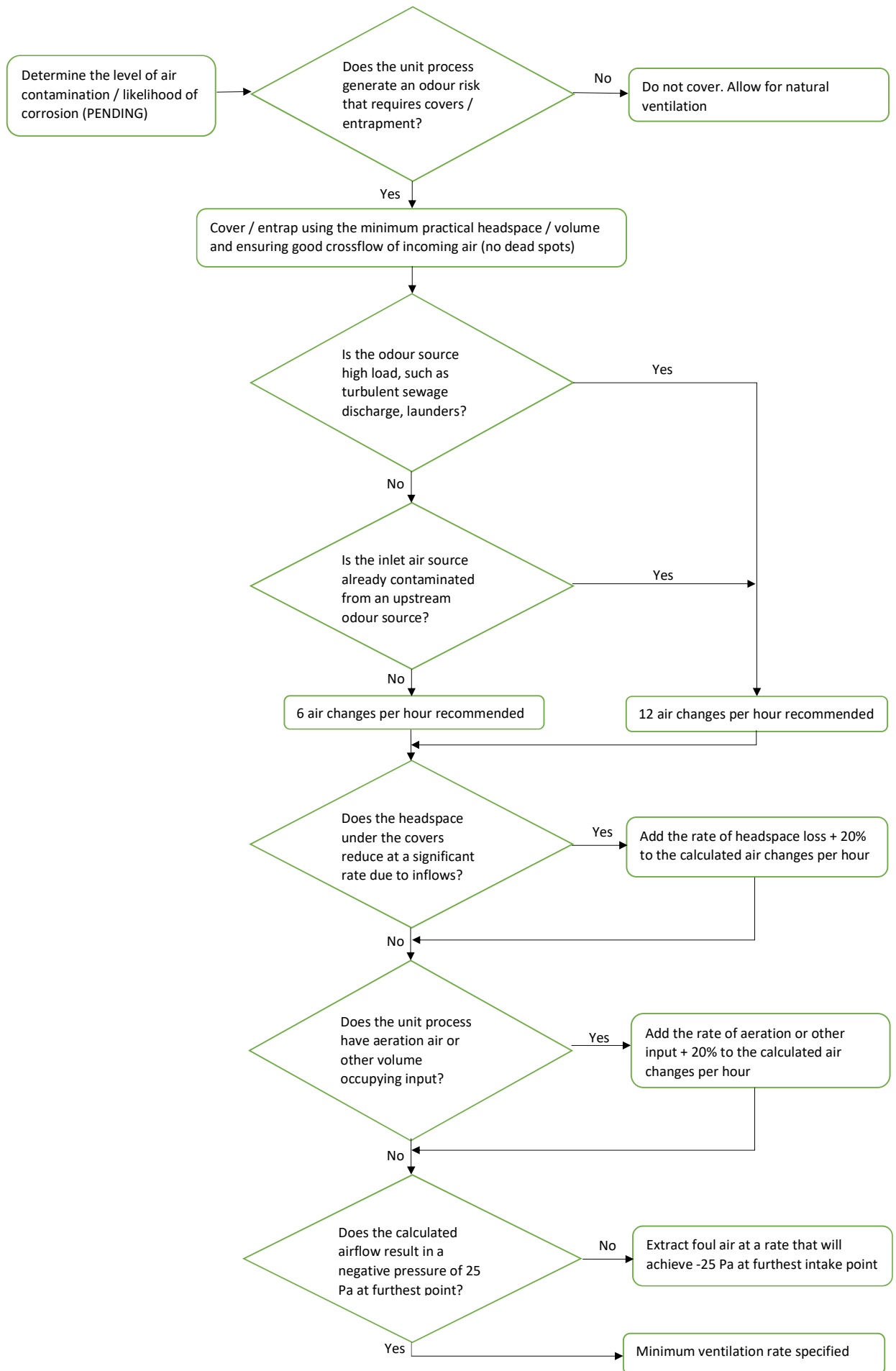
Figure 1 – Minimum Airflow Flowchart Treatment Processes
