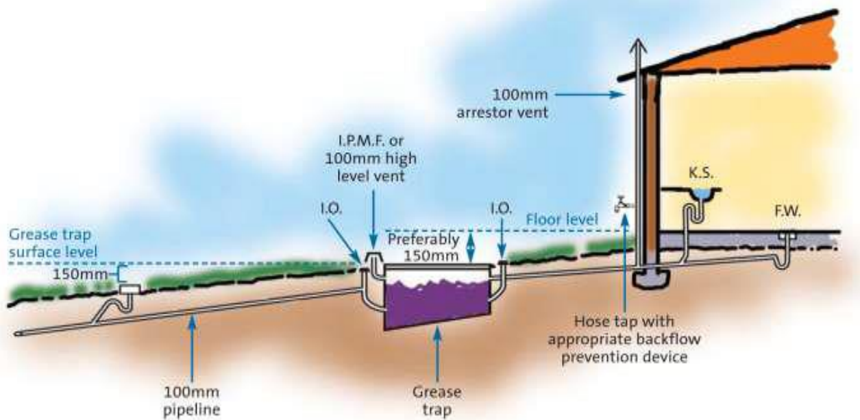
Preferred drainage layout for a grease trap installation
